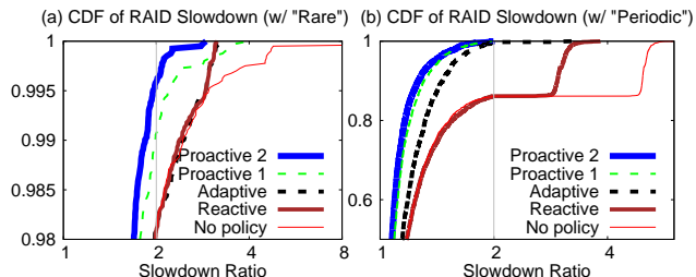
Figure 12: TolerRAID evaluation. The figures show the pros and cons of various TolerRAID strategies based on two slowdown distributions: (a) Rare and (b) Periodic. The figures plot the T^1 distribution (i.e., the RAID slowdown). T^1 is essentially based on the longest tail latency among the necessary blocks that each policy needs to wait for.
